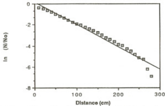
Fig. (2): Natural logarithm of fraction of ants still following the path as a function of distance; linear trail; \ln(N/N_0) = 0.197 - 0.021r ; r =distance;
