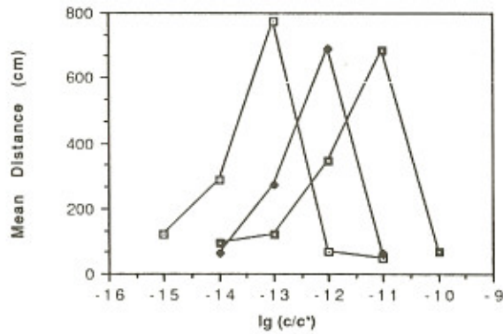
Fig. (3): Mean trail distance followed as a function of the amount of pheromone ; linear trail; Ref values: \square = 5 \times 10^{-13} \text{ g/cm}^3 ; \diamond = 5 \times 10^{-12} \text{ g/cm}^3 ; \triangle = 5 \times 10^{-11} \text{ g/cm}^3 ; Parameters: idem fig.(2), except: number of ants used for each simulation = 100; equiprobable distribution of starting angles
