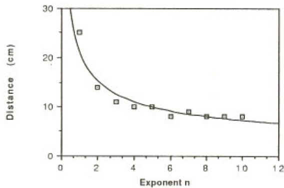
Fig.(4): Mean trail distance followed as a function of the flexibility exponent n; linear trail; Parameters: idem fig.(2), except: SI = 0.35 \text{ cm} ; equiprobable distribution of starting angles
