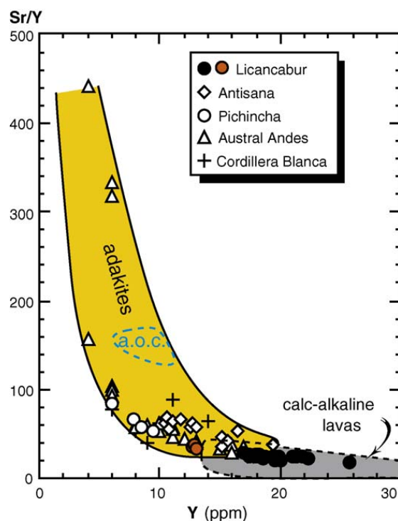
Fig. 5. Y—Sr/Y diagram for Licancabur lavas. Selected lavas from Antisana [3], Pichincha [2], AVZ [27] and granodiorites from the Cordillera Blanca batholith, Peru, [24] are also plotted. Fields for adakites and calc-alkaline lavas [6], and for experimental melting of altered oceanic crust (aoc) [26] are indicated.
