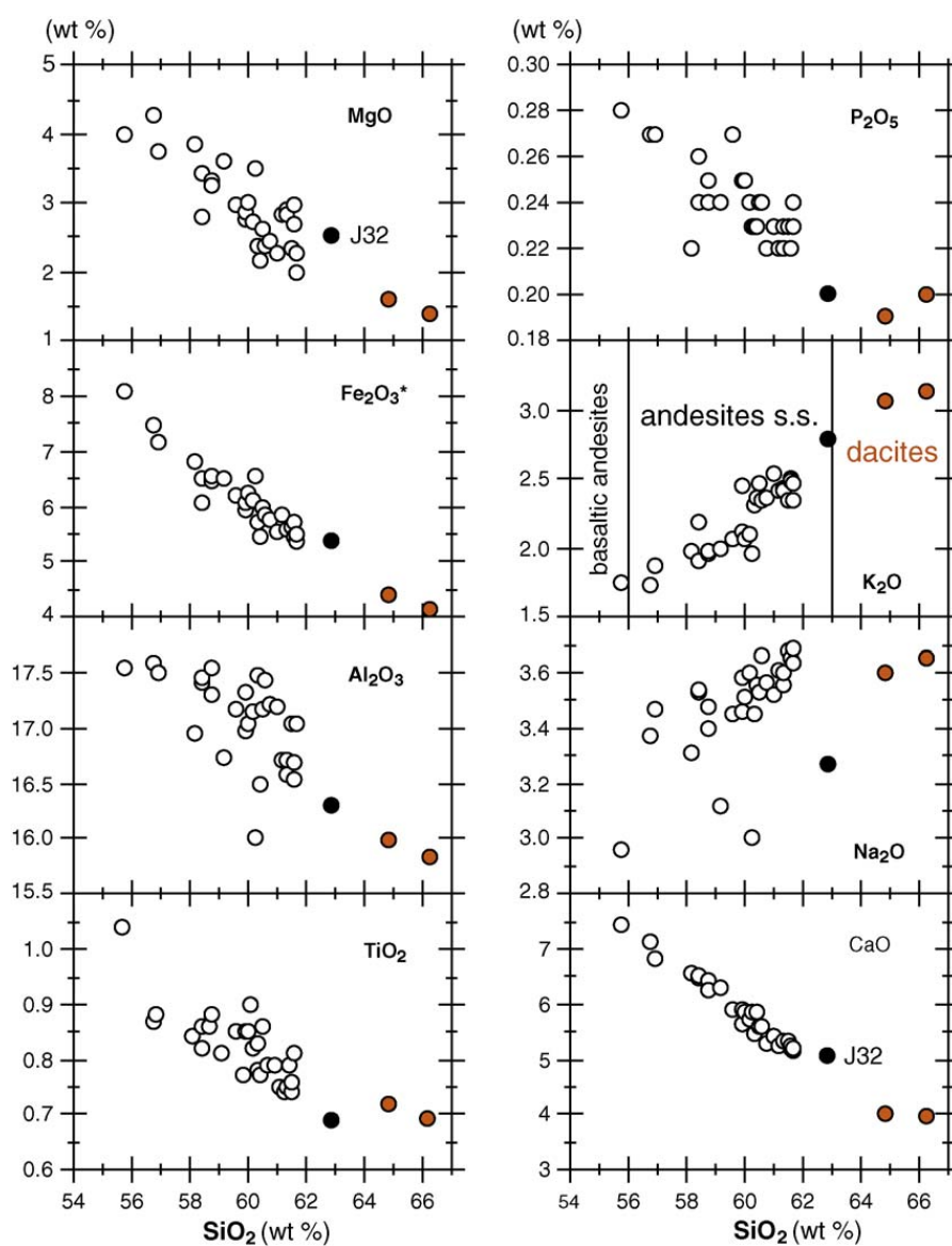
Fig. 2. Harker diagrams for Licancabur lavas. The nomenclature of the lavas is indicated in the SiO 2 –K 2 O diagram. Purico ignimbrite J32 is also plotted.
