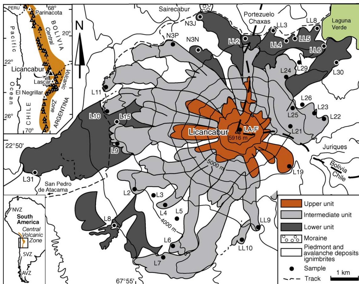
Fig. 1. Location of Licancabur volcano in the Andean Central Volcanic Zone. Lower inset: the four Andean volcanic zones (NVZ: 5°N–2°S, CVZ: 14°S–27°S, SVZ: 33°S–46°S, AVZ: 49°S–55°S, northern, central, southern, and austral Volcanic Zones, respectively). Upper inset: the main volcanoes of the CVZ south of 17°S.
