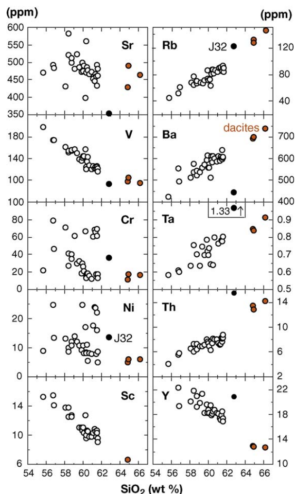
Fig. 3. Trace element distribution in Licancabur lavas according to their \text{SiO}_2 content. Purico ignimbrite J32 is also plotted.
