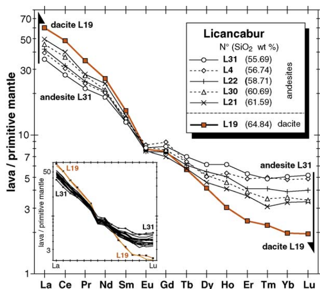
Fig. 4. Primitive mantle [23] rare earth normalized abundance diagram for Licancabur representative lavas. The silica contents of the selected samples (wt %) are indicated. Inset: patterns for studied Licancabur lavas.
