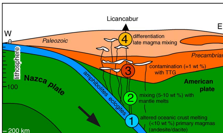
Fig. 6. Model of genesis of Licancabur lavas (see text for explanations).
