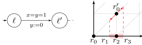
Figure 5: Perturbing one transition.
