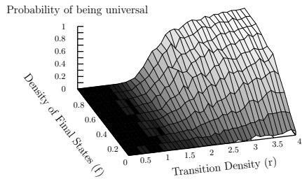
Fig. 2. Probability of universal automata ( |\text{Loc}| = 30 ).
