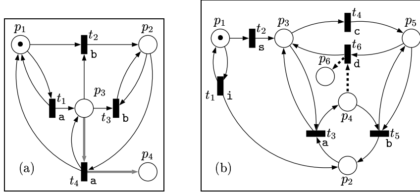
Figure 2: (a) The PN+T \mathcal{N}_1 and (b) the PN+NBA \mathcal{N}_2 .
