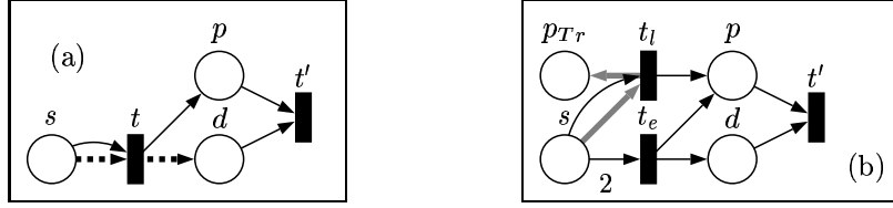
Figure 1: A PN+NBA \mathcal{N} (a) and the corresponding PN+T \mathcal{N}' (b)
