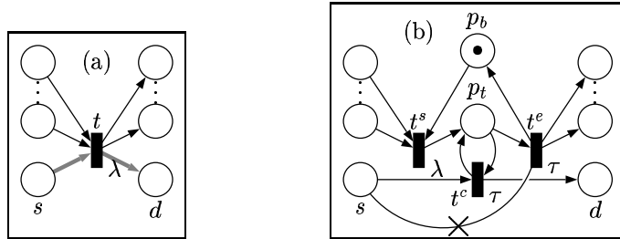
Figure 3: How to transform a PN+T (left) into a PN+R (right). The edge bearing a \times links the (source) place to be reset to the extended transition. p_{T_r} is not shown.
