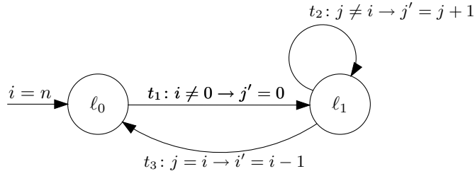
Fig. 5. Our two counters automata modeling the Bubblesort algorithm
