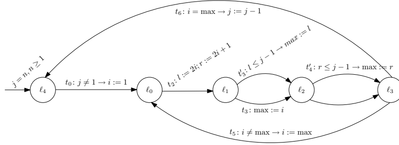
Fig. 4. Counters automata modeling of the Heapsort algorithm
