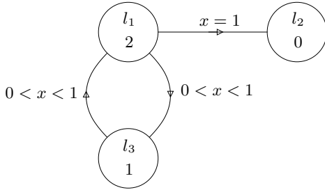
Fig. 8. A weighted timed automaton
