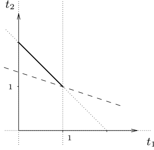
Fig. 4. Optimizing the cost of \rho_1(t_1, t_2)
