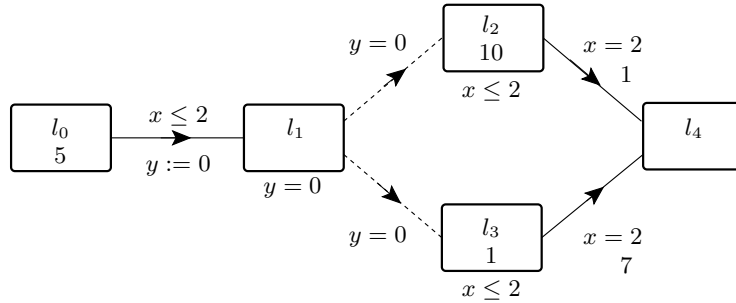
Fig. 20. A weighted timed automaton inspired from [BCFL04]
