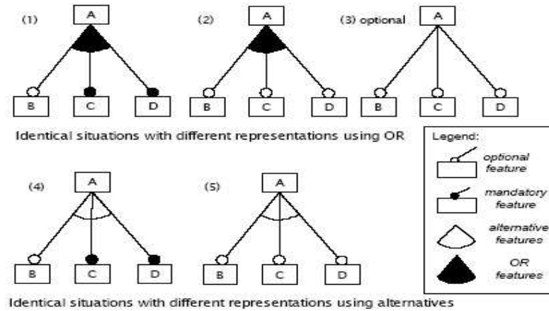
Fig. 9. Ambiguity example [13]
